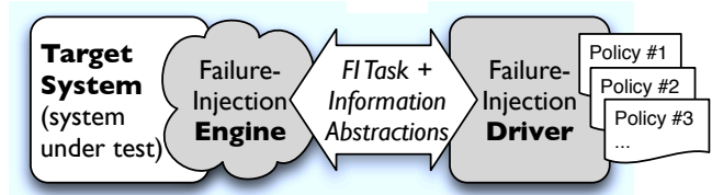
Figure 2. PREFAIL Architecture. The figure shows the separation of failure-injection engine (mechanism) and driver (policy). The pruning policies written in the driver make failure decisions that drive the engine.
